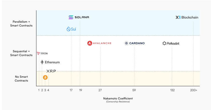
Figure 2: Comparison of the decentralization and censorship resistance of blockchains, as measured by the Nakamoto Coefficient, alongside their parallel processing and smart contract capabilities.
