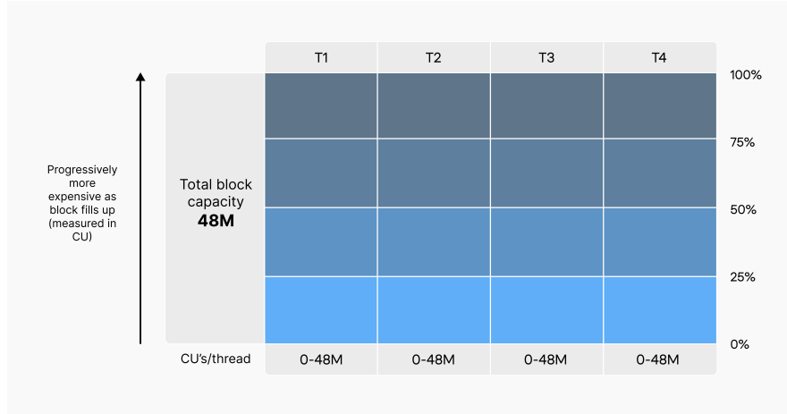
Figure 5: Visualization of X1 Blockchain's dynamic base fee mechanism. The fee increases progressively as the block fills up, with block capacity measured in Compute Units (CU) across threads.
