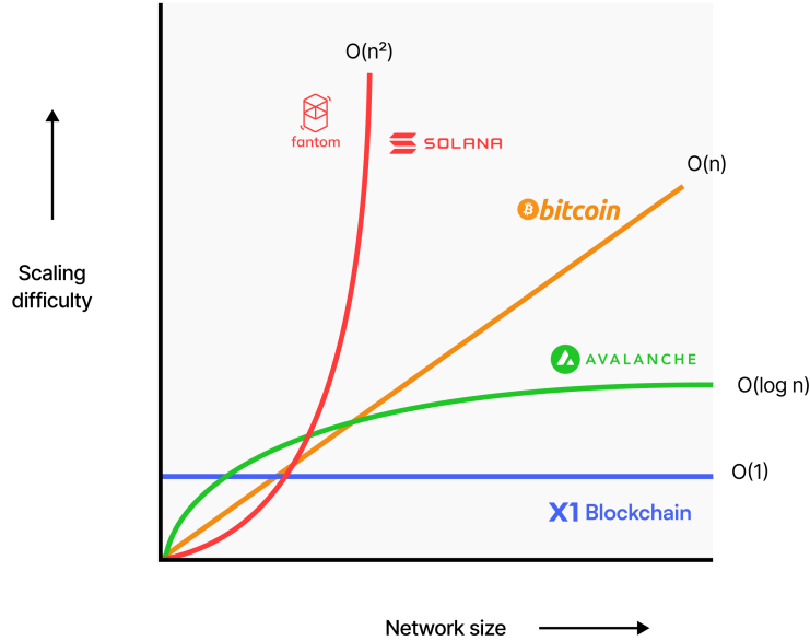
Figure 4: Comparison of how different blockchains scale based on Big O Notation. X1 Blockchain achieves O(1) complexity, indicating minimal scaling difficulty with increasing network size, while other chains such as Solana and Fantom face O(n^2) complexity.
