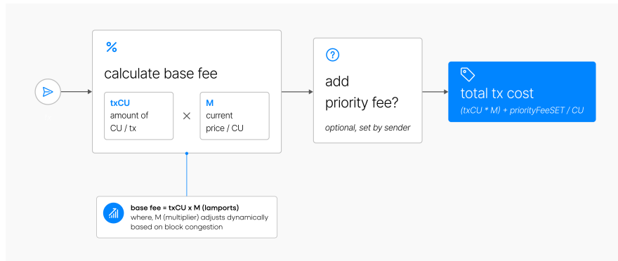
Figure 6: Diagram illustrating how transaction fees are calculated on X1 Blockchain. The total transaction cost is determined by the base fee ( \text{txCU} \times M ) and an optional priority fee set by the sender.
