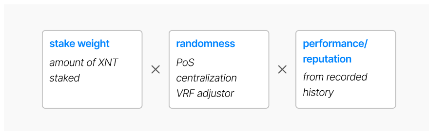
Figure 3: Factors determining block production eligibility on X1 Blockchain. These include stake weight, randomness (via VRF), and performance/reputation from recorded history.
